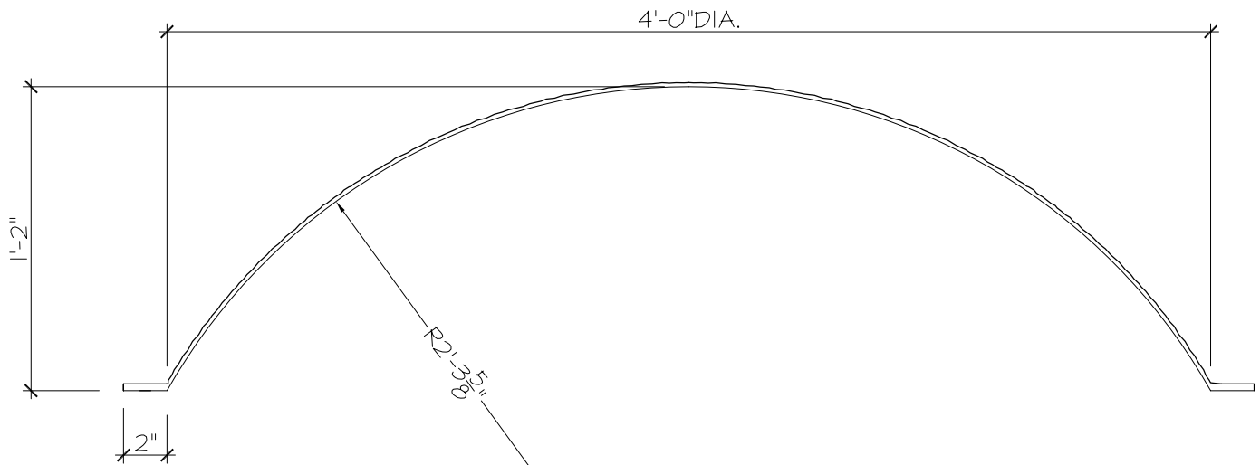
1A REFLECTED PLAN VIEW SCALE : 3/4" = 1'-0"
