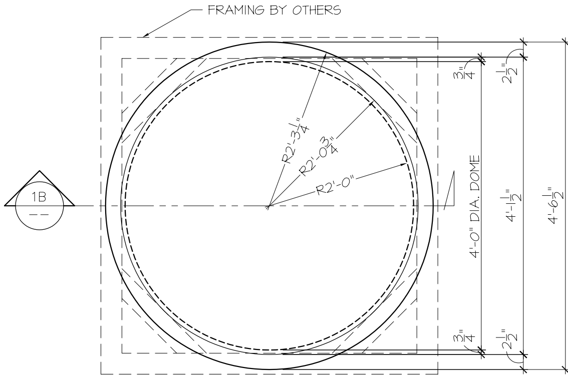
1A REFLECTED PLAN VIEW SCALE : 3/4" = 1'-0"
