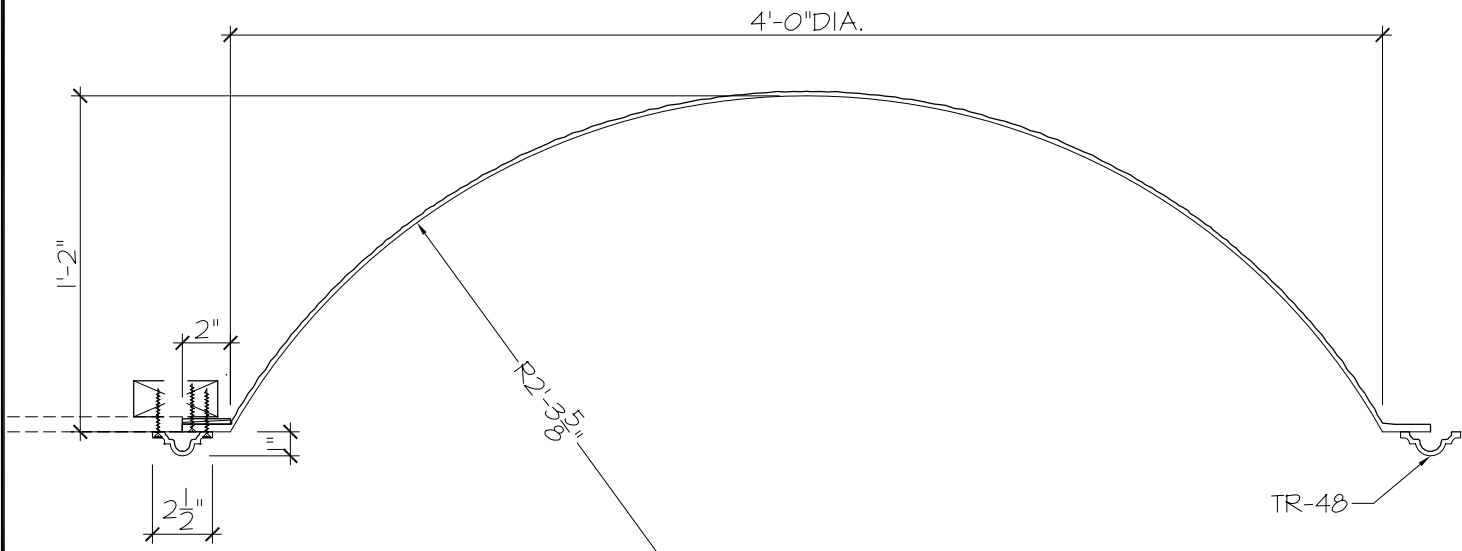
1B DETAIL SECTION SCALE : 1-1/2" = 1'-0"
